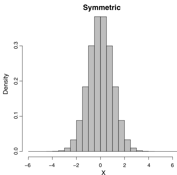
Fig. 2.12 An example of a symmetric histogram
