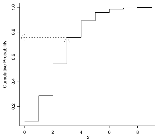
Fig. 5.17 Plot of the cdf for a Poisson distribution with \mu = 2.5 . By following the arrows from x = 3 to the cumulative probability, we can obtain the lower tail probability of observing three or fewer physician visits per year: P(X \leq 3) = 0.75
