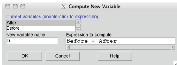
Fig. 8.6 Computing the difference variable D in R-Commander
