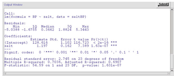
Fig. 11.9 Output of fitting a linear regression using R-Commander for investigating the relationship between blood pressure (BP) and sodium chloride intake (salt)
