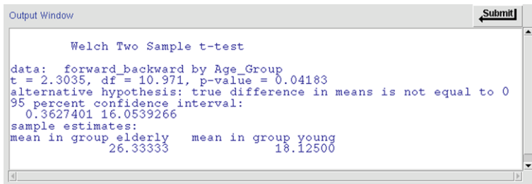
Fig. 8.4 The results of two-sample t -test for the balance example. The t -score is 2.3, the degrees of freedom for the t -distribution is 10.97, and the corresponding p -value is 0.042. The 95% confidence interval is [0.36, 16.05]
