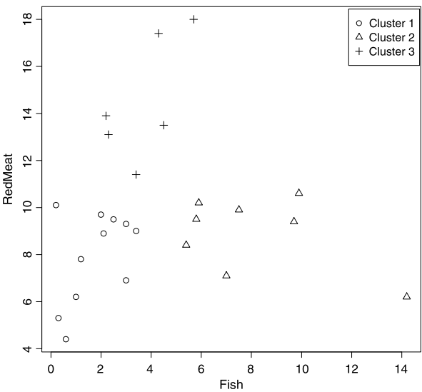
Fig. 12.4. The first cluster is represented by circles and contains countries whose consumption of both fish and red meat is relatively low. The second cluster is represented by triangles and includes countries whose consumption of both fish and
