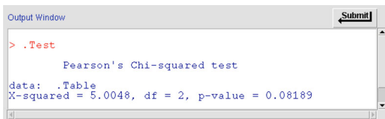
Fig. 10.7 Results from the \chi^2 test of independence for the relationship between race and low. The test statistic is q = 5.0 , and using the \chi^2 distribution with 2 degrees of freedom, the resulting p -value is 0.08
