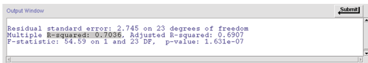
Fig. 11.10 Measures of goodness of fit provided by R-Commander for linear regression models. Here, our model uses salt as the explanatory variable for BP . For this model, R^2 = 0.70
