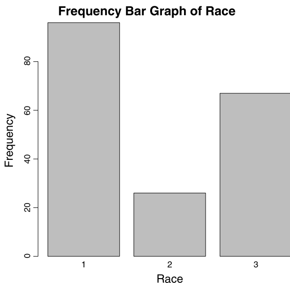
Fig. 2.6 Bar graph for mother's race in the birthwt data set, where 1, 2, and 3 represent the categories "white", "African-American", and "other", respectively
