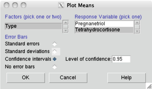
Fig. 9.6 Creating a plot of means for the Tetrahydrocortisone by syndrome type from the Cushings data set. Here, we choose Confidence intervals at 0.95 level of confidence for Error Bars. This way, R-Commander shows the 95% confidence interval around the sample mean for each group
