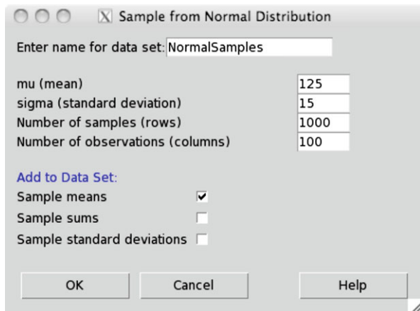
Fig. 6.3 Using R-Commander for simulating samples from the population, measuring \bar{X} , and calculating \bar{x} . Here, we are generating 1000 samples of size n = 100 from N(\mu = 125, \sigma = 15) distribution
