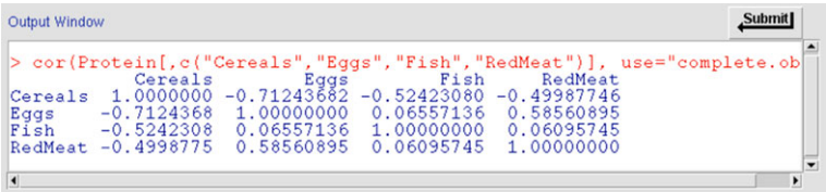
Fig. 3.6 Correlation matrix for most of the numerical variables in the Protein data set
